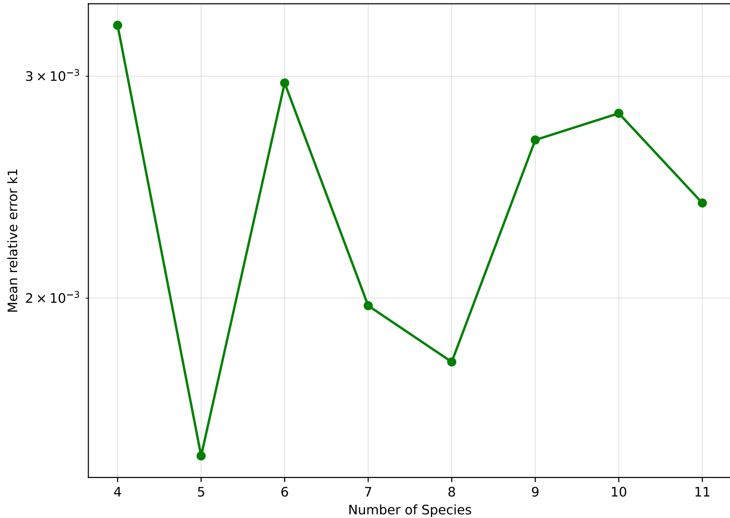
30, 30, 30 — Mean relative error k1 vs number of species (zoomed: 4 to 11 species)
